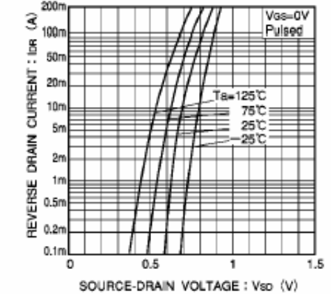
Fig.9 Reverse drain current vs. source-drain voltage ( I )
